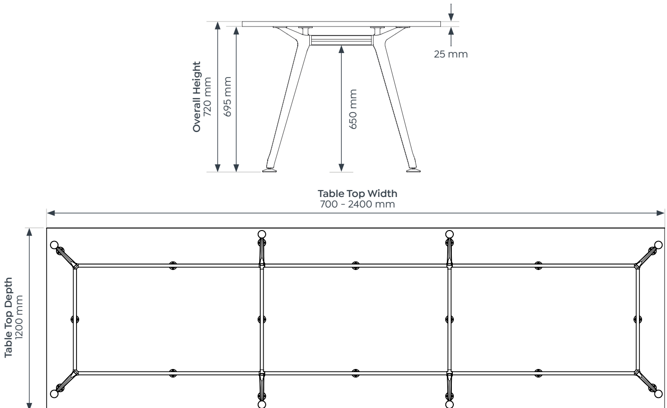
Team Table - 8 Leg (Typical Frame Dimensions)
