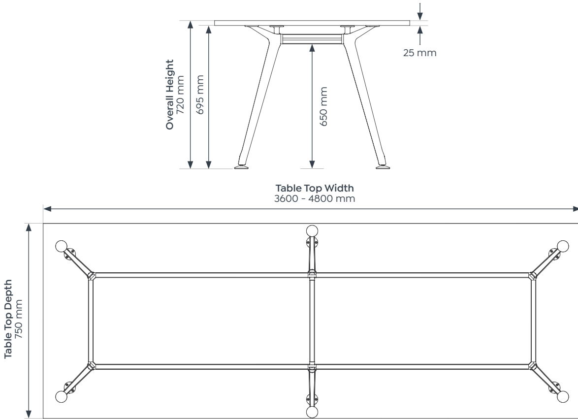
Team Table - 6 Leg (Typical Frame Dimensions)
